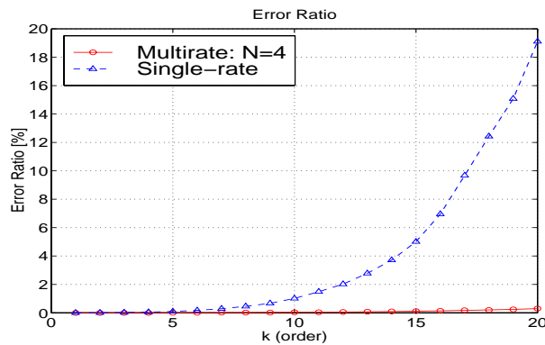
Figure 6.7: Error ratio E_R(k) . (20th order corresponds to 2.4 [kHz].)
