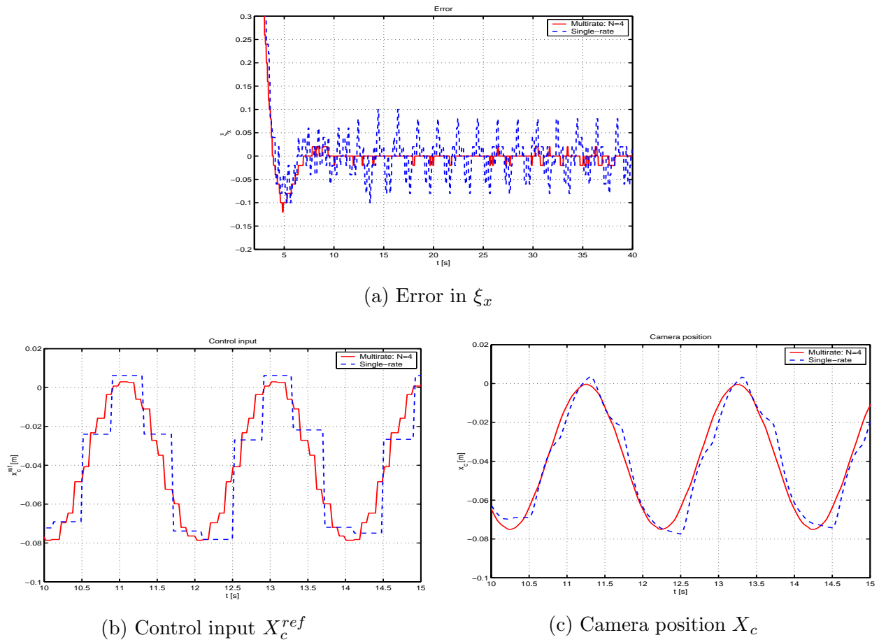
Figure 6.16: Experimental results ( T_y = 400 [ms], N = 4 ).
