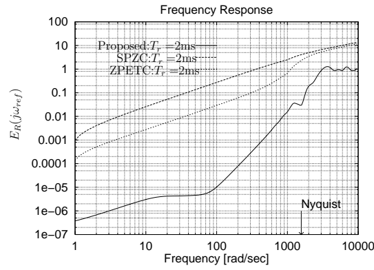
Figure 5.7: Frequency responses of the intersample tracking error. (The error ratio (5.4) vs. frequency of the desired trajectory \omega_{ref} )
