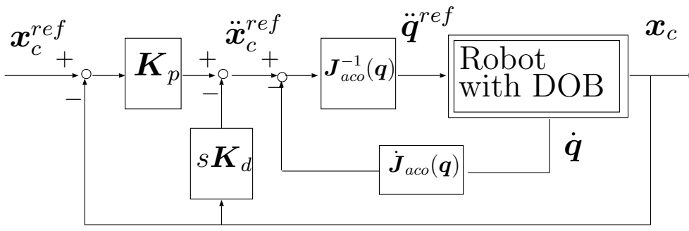
Figure 6.11: Workspace controller (inner-loop).
